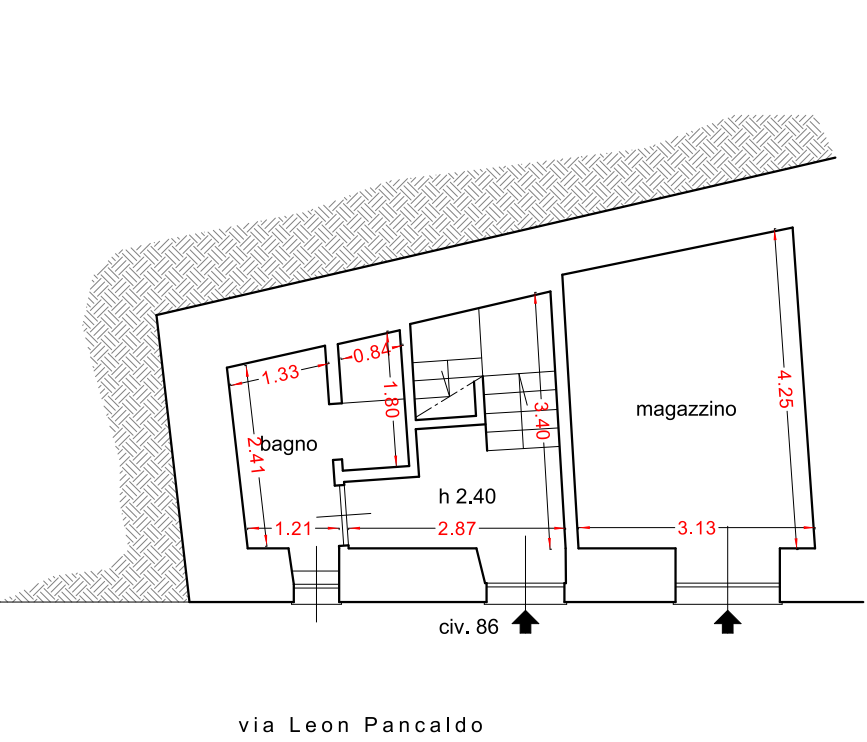
PIANO TERRA
